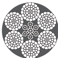
6xK49SF+IWRC (plastic filled)
