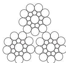
6x19S (9-9-1)
